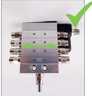
Figure 5: Mounting position hanging, rotated 180°
