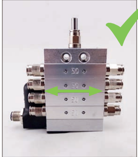
Figure 4: Mounting position hanging, piston horizontal
