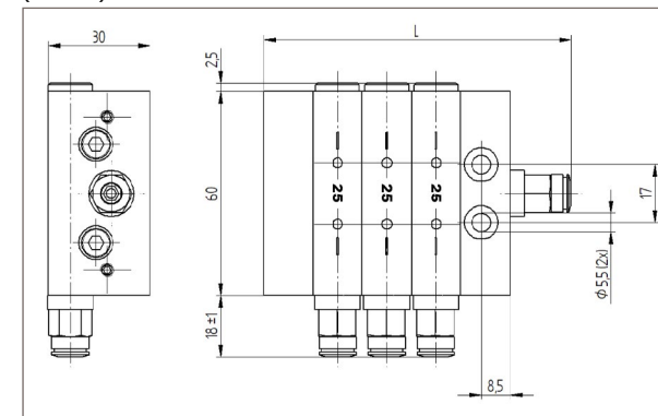
Figure 2: Dimensions PRV-3
