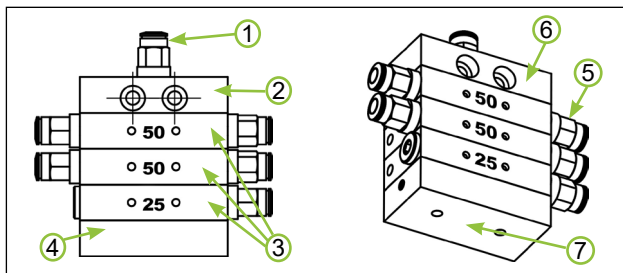
Figure 1: Overview PRV-5
