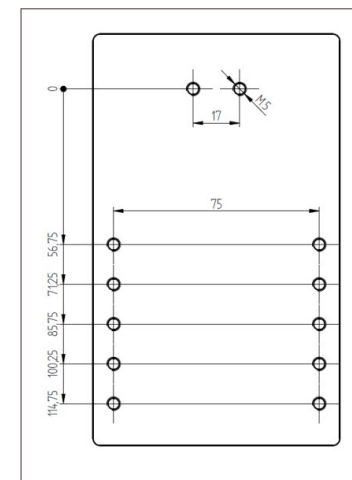
Figure 3: Drilling pattern
